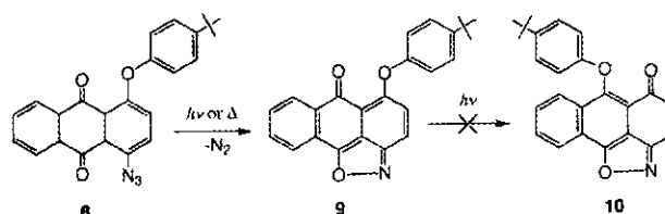
Scheme 3. Synthesis of 9 .
