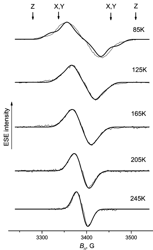
Figure 3. Thin lines: the experimental echo-detected EPR spectra of {}^3\text{C}_{60} in o -terphenyl glass at different temperatures measured at \tau = 120 ns. Thick lines: simulated spectra (see text). Spectra are arbitrarily shifted along the vertical axis. The arrows mark the field position corresponding to the canonical orientations of {}^3\text{C}_{60} in the absence of motion.
