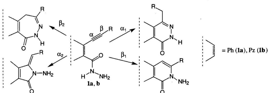
Scheme 1. The four possible routes of cyclization of hydrazides derived from acetylenylbenzoic ( 1a ) and pyrazolecarboxylic ( 1b ) acids.
