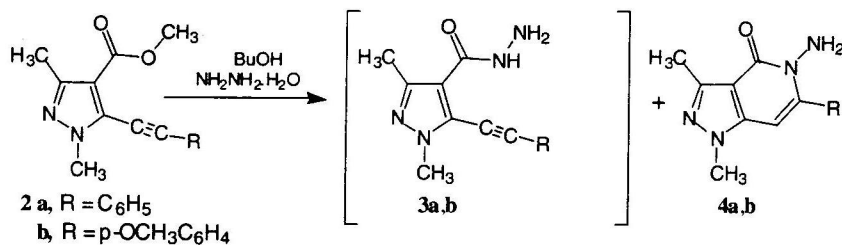
Scheme 2. Hydrazinolysis of methyl esters 2a and b .
