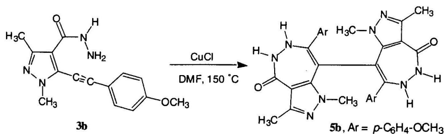
Scheme 3. The unexpected formation of the pyrazolodiazepinone 5b .
