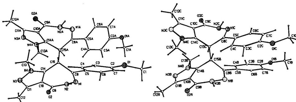
Figure 1. View of two crystallographically independent molecules of 5b and numbering scheme.
