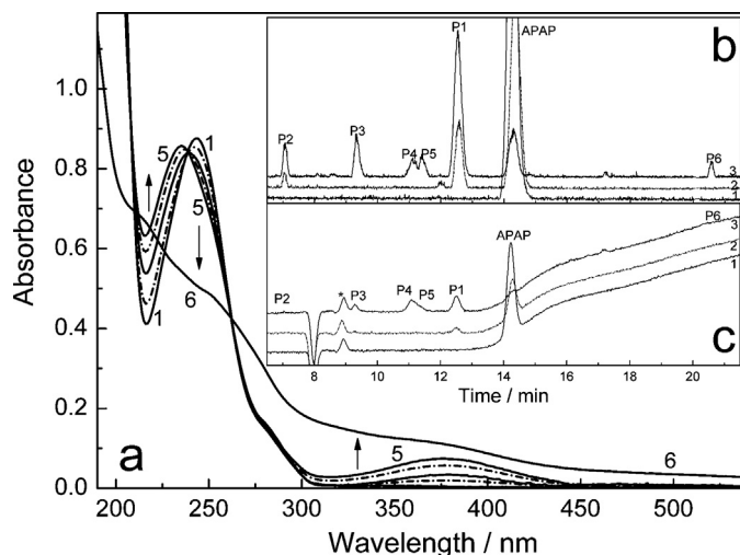
Fig. 4. Optical spectra (a) of air-saturated APAP ( 8.3 \times 10^{-5} M) solution after 0 (1), 7 (2), 20 (3), 30 (4), 40 (5) and 200 (6) min of irradiation at 254 nm. The base peak (b) and UV (c) chromatograms after 0 (1), 20 (2) and 200 (3) min of irradiation, accordingly. *Impurity in the eluent. The energy of excitation was 6 \times 10^{-4} \text{ E} \times \text{l}^{-1} \times \text{min}^{-1} .
