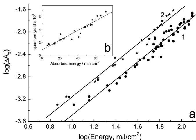
Fig. 3. (a) The dependence of the hydrated electron ( \lambda_{\text{reg}} = 720 nm, argon-saturated solutions) and RO• ( \lambda_{\text{reg}} = 440 nm, air-equilibrated solutions) yields on laser excitation energy in log–log coordinate. The slope of both lines is 1.6. (b) The dependence of the observed quantum yield of the hydrated electron on excitation energy.
