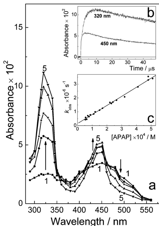
Fig. 2. (a) Transient absorption spectra recorded 0.05 (1), 0.4 (2), 1.6 (3), 4 (4) and 9.6 (5) μs after the laser excitation of K 2 S 2 O 8 (0.04 M) in the presence of APAP (6.5 × 10 -5 M). (b) Characteristic kinetic curves at 320 and 450 nm. (c) The dependence of the observed rate constant of RO• radical formation at 320 nm on concentration of APAP.
