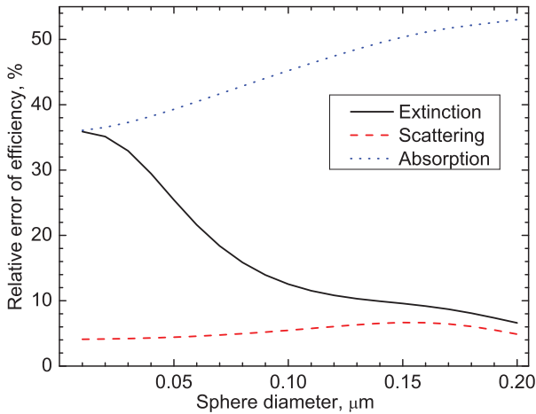
Figure 2.5 Relative errors of Q_{ext} , Q_{sca} , and Q_{abs} of a gold sphere computed using the FCD formulation of the DDA as a function of sphere diameter ( \lambda = 0.694 \mu\text{m} , N_x = 64 ).
