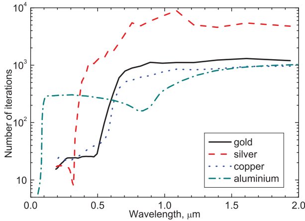
Figure 2.2 Estimated number of iterations, based on Eq. (2.37), for DDA simulations of metallic nanoparticles (in vacuum) in logarithmic scale.
