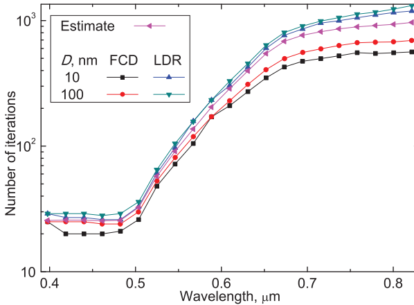
Figure 2.1 Number of iterations for DDA simulations of gold nanospheres (in vacuum) in logarithmic scale. Real data is for two diameters D and two DDA formulations (see Sec. 2.4.3); estimate is based on Eq. (2.37).
