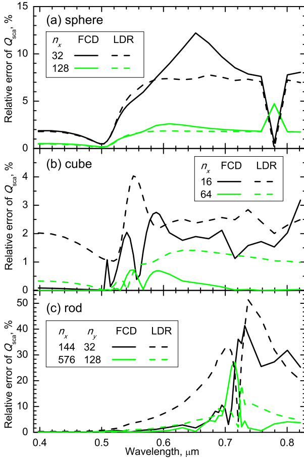
Figure 2.4 Same as Fig. 2.3 but for scattering efficiency Q_{sca} .
