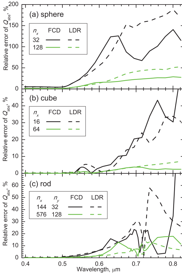
Figure 2.3 Relative errors of absorption efficiency Q_{abs} computed using the FCD and LDR formulations of the DDA, varying the number of dipoles, for gold (a) 10-nm sphere, (b) 10-nm cube, and (c) 20 \times 90 -nm rod.
