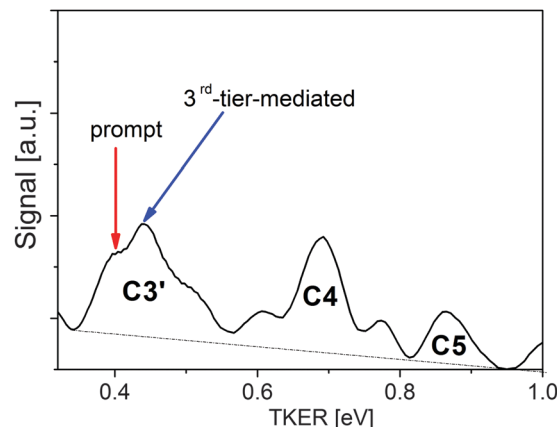
Fig. 9 Example of the distribution of TKER values for \text{I}^+ ions arising in channel C3' due to electron photodetachment from a wavepacket propagating in the 1st tier IP state. The presented data are measured at a delay time of 6.67 ps. The red arrow indicates the maximum of TKER values expected for the case when wavepacket propagation in the 1st tier state starts at the moment of excitation (prompt predissociation via 1st tier state); the blue arrow shows the case of predissociation via the 1st tier state when propagation starts with a delay of 1600–1700 fs which roughly matches the oscillation period of the 3rd tier state (3rd-tier-mediated, see text).
