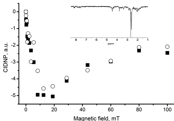
Fig. 1 CIDNP field dependence (low field region) for N-CH 3 protons (2.6 ppm) measured after laser irradiation (308 nm) of 2 mM solutions of the ( R,S )- (■) and ( S,S )-NPX-PYR (○) dyads in ACN ( \epsilon = 37.5 ). The inset shows the CIDNP effects of N -methyl pyrrolidine protons in the ( S,S )-NPX-PYR dyad detected in a magnetic field of 12.5 mT.
