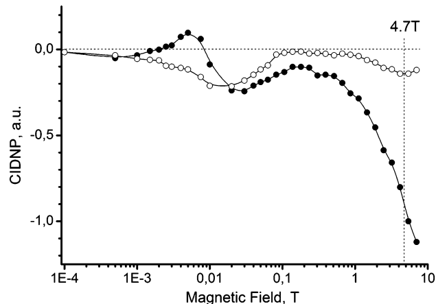
Fig. 8 CIDNP field dependence of N-CH 3 protons measured after laser irradiation (308 nm) of 2 mM solution of the (R,S)-NPX-PYR dyad in ACN (O, \epsilon = 37.5 ) and a ACN/BZ mixture (●, \epsilon = 10 ) on the external magnetic field strength ( B ). The ratio of field dependence at 4.7 T corresponds to the literature values reported for the CIDNP dependence on solvent permittivity. 11
