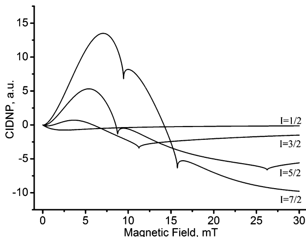
Fig. 5 Calculated dependence of CIDNP for the product from RPs with different values of nuclear spin I on the magnetic field strength at a HFI constant a = 3 mT.
