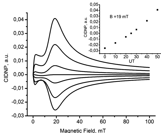
Fig. 4 Calculated CIDNP field dependence for RP with one magnetic nucleus with spin I = 3/2 for different contributions of recombination from the singlet and triplet states ( U_S + U_T ) \tau_r = 0.5 . From the bottom to top – U_T\tau_r = 0, 0.1, 0.2, 0.25, 0.3, 0.4, 0.5 . Inset – the value for CIDNP at a magnetic field of 19 mT from the contribution of the triplet recombination channel ( U_T\tau_r ).
