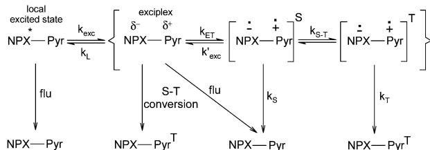
Scheme 1 Quenching of the excited singlet state of the NPX-Pyr dyad. The following symbols are used to describe the rate constants of separate stages: k_{\text{exc}} – local excited state transfer to exciplex; k_L – transfer of exciplex to local excited state; k_{\text{ET}} – electron transfer; k'_{\text{exc}} – transfer from biradical ion to exciplex; k_{\text{S-T}} – singlet-triplet conversion in biradical ion; flu – fluorescence quenching; k_S and k_T – back electron transfer from the singlet and triplet spin states of biradical ion.
