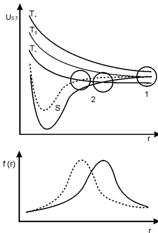
Fig. 7 At the top – the dependence of the singlet and triplet energy levels of the biradical on the distance between the radical centers. The two transition zones 1 and 2 correspond to the area of weak and the strong exchange interaction, respectively. At the bottom – the probability of the distance distribution between the radical centers in the biradical at different permittivities: the solid line corresponds to high permittivity and dotted line refers to low permittivity.
