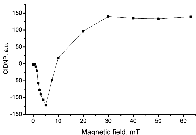
Fig. 3 CIDNP field dependence (low field region) for N-CH 2 protons of TEA measured after laser irradiation (308 nm) of 2 mM solution of naphthalene in the presence of 10 mM TEA in CD 3 CN.
