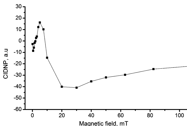
Fig. 2 CIDNP field dependence for N-CH 3 protons measured after laser irradiation (308 nm) of 2 mM solution of the ( R,S )-NPX-PYR dyad in a ACN/BZ mixture at \epsilon = 10 .
