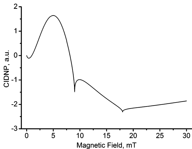
Fig. 6 Calculated dependence of CIDNP of the product from RP containing 6 equivalent protons on the magnetic field strength at a HFI constant a = 3 mT.
