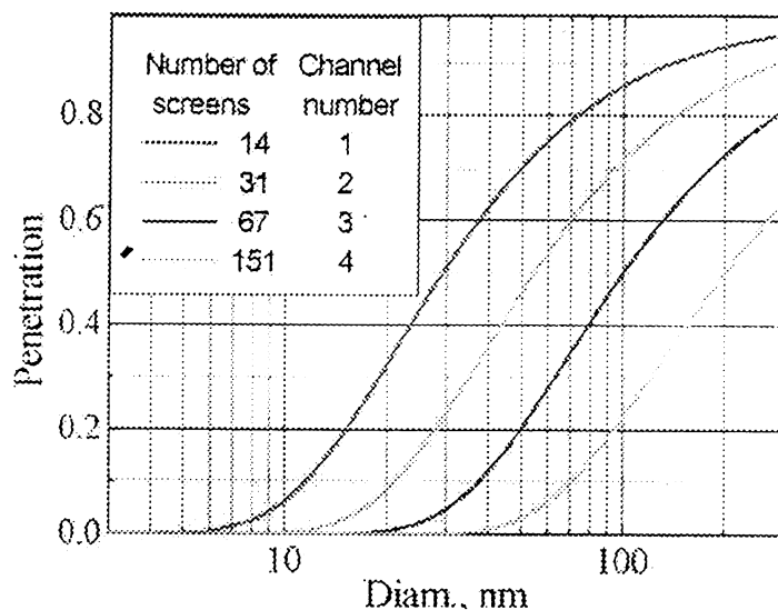
Figure 2. Calculated calibration efficiency of penetration of particles by four cascades of the diffuse cutter (airflow rate is 4 l/min).
