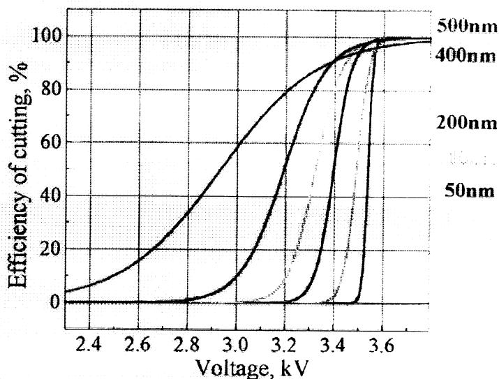
Figure 4. Cutting efficiency of electrostatic filter for 50–500 nm particles.
