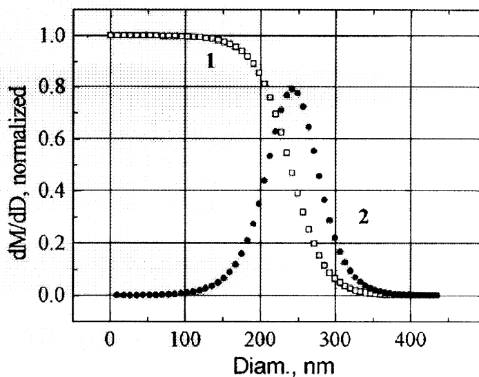
Figure 5. Preliminary results for experimental mean soot size distribution: 1) integral curve (measurements, fitting), 2) calculated soot size spectrum.
